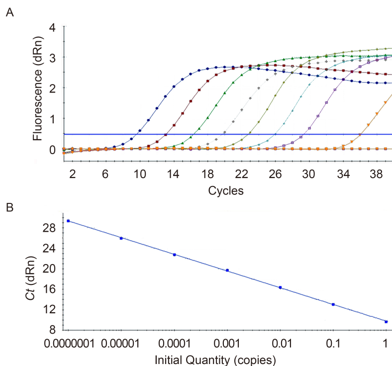
Supplementary Figure S1. The amplification plots (A) and standard curve (B) constructed by serial 10-fold dilutions of the standard plasmid pMD-DENV 2 .
