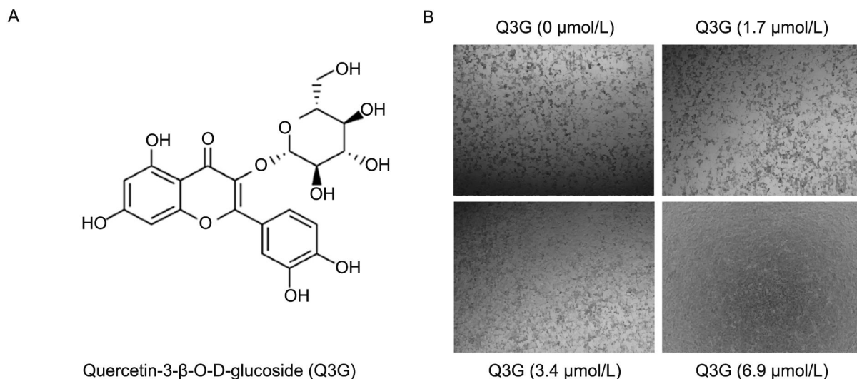
Figure S1. (A) Chemical structure of quercetin-3- \beta -O-D-glucoside (Q3G). (B) Inhibitory effect of Q3G at the indicated concentrations of ZIKV PLCa1_ZV (MOI = 0.05) in Vero cells, as visualized under a microscope (at 4x magnification) at 4 dpi.
